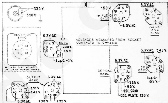
Fig. 1—Socket Voltages—Underside of Chassis View
