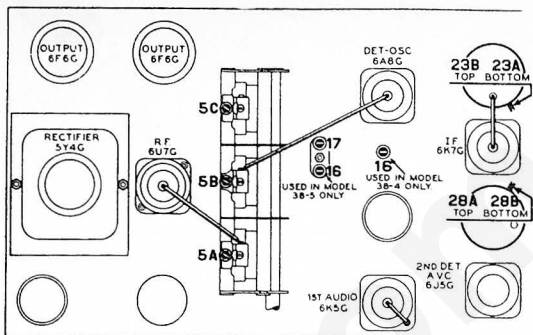
Fig. 5. Locations of Compensators--Top of chassis
