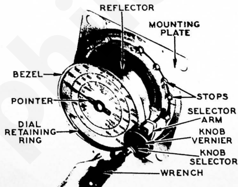
Fig. 2—Cone-Centric Automatic Tuning Mechanism, Model 4
