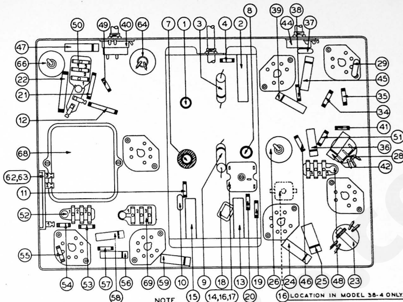
Fig. 4—Locations of Parts, Underside of Chassis
